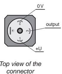
3-wire connection scheme CLS-53N-P(N)
