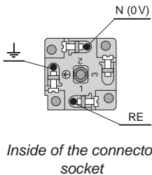
2-wire connection scheme CLS-53N-SAC
